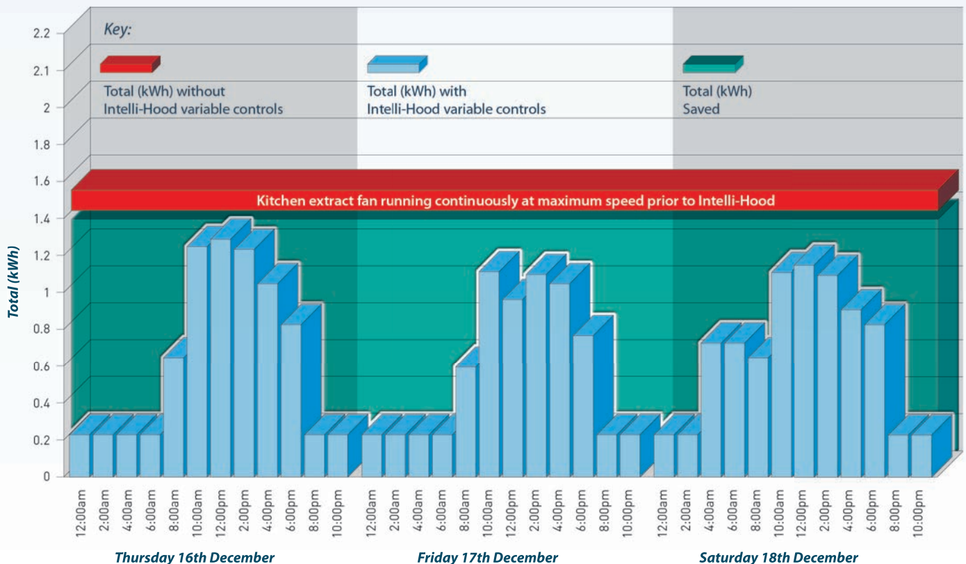
3 day comparison graph for Asda Rotisserie Counters with percentage of energy saved.
